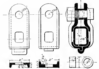
Figs. 1587-1593. WHEEL-GUARD FOR KEWANEE STEEL BRAKE-BEAM.
